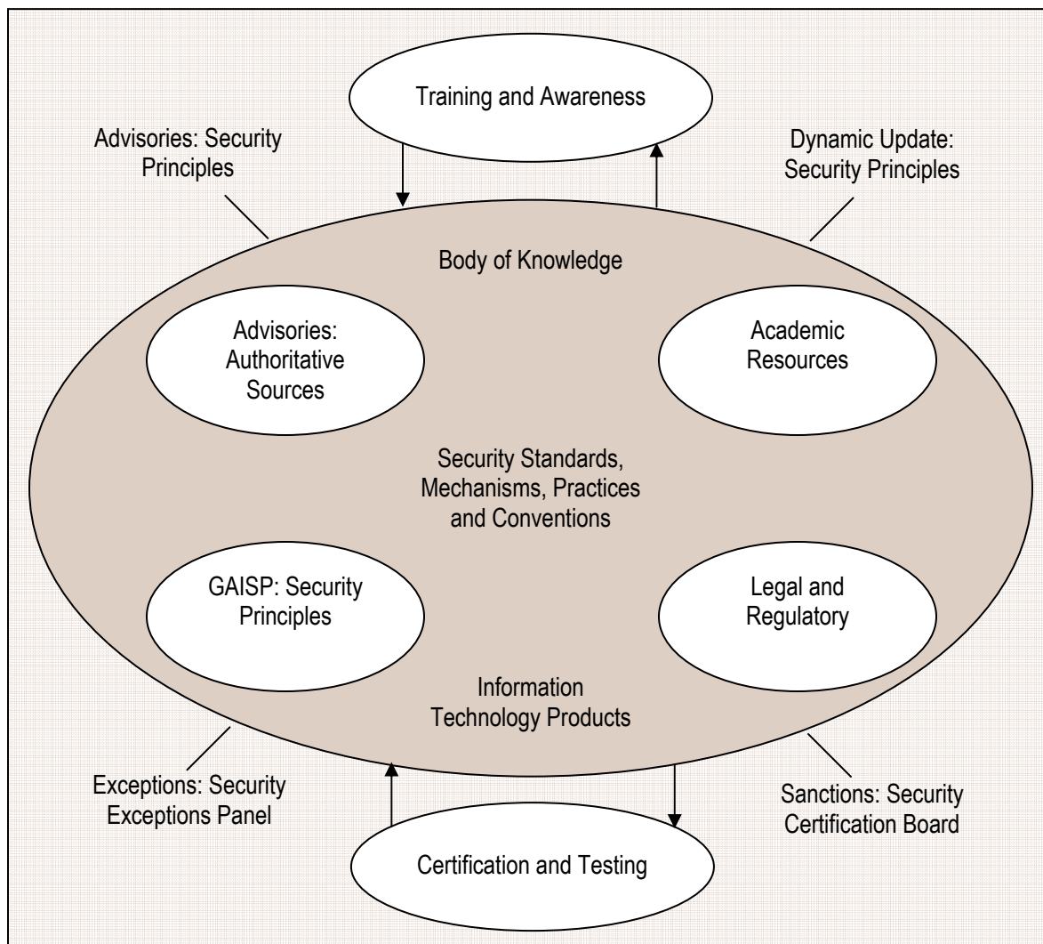
Figure Error! No text of specified style in document.-1: Role of GAISP and Product Profiles in Relation to Information Systems Security Certification and the Body of Knowledge
